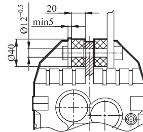
GFA37-T
