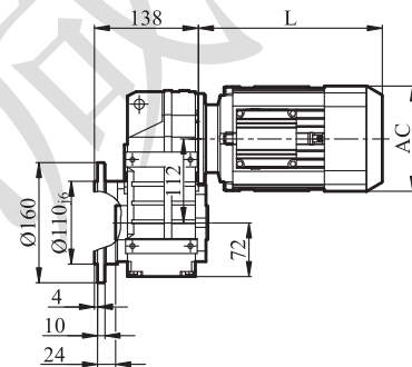
GFAF/GFHF/GFVF37
