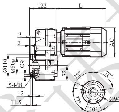
GFAF/GFHF/GFVF37
